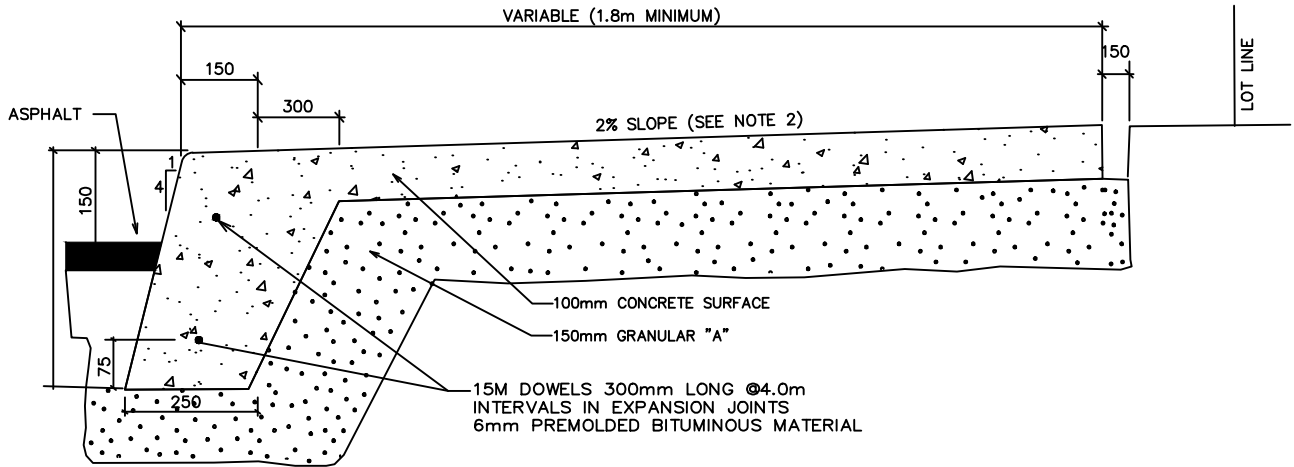
TYPICAL SIDEWALK SECTION
