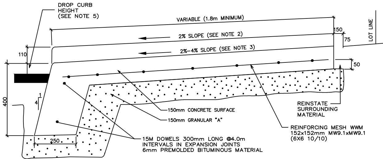
SECTION AT PEDESTRIAN AND ENTRANCE RAMP
