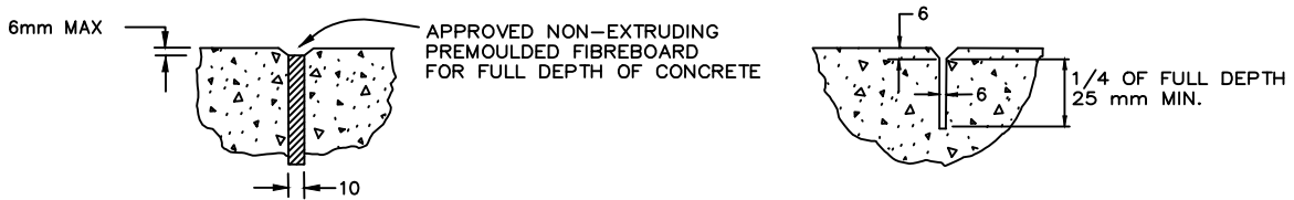
EXPANSION JOINT PROFILE DUMMY JOINT PROFILE
